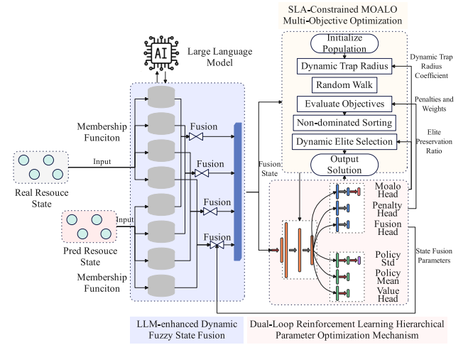
Fig. 1 The framework of LFRL-MOS
