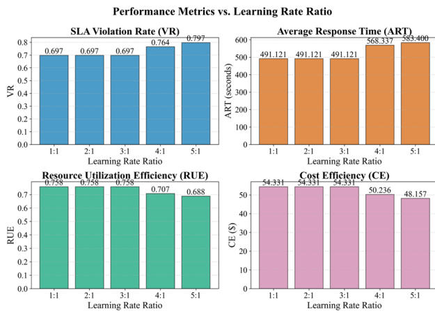
Fig. 4 Performance Metrics of Different Learning Rate Ratio
